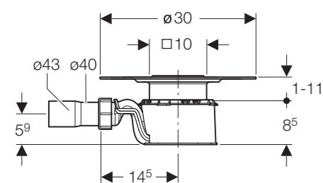
Drain for flat showers 154.005.00.1
